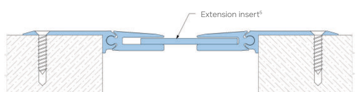
5 Profiles for a joint width of 130 mm are completed with an extension insert: - SV 42/130, SV 42/150, SV 42/170, SV 42/200
